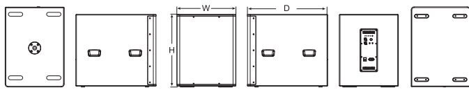
Dimension(W×H×D): 510×632×695mm
